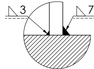
DETAIL A SCALE 2 : 5
