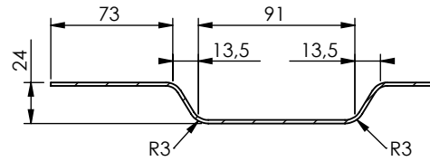
DETAIL B SCALE 1 : 4
