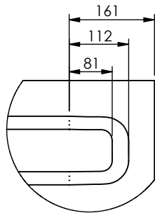
DETAIL A SCALE 1 : 10
