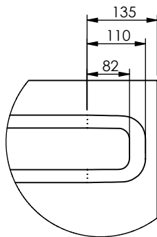
DETAIL A SCALE 1 : 10
