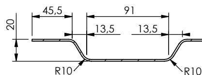
DETAIL B SCALE 1 : 4
