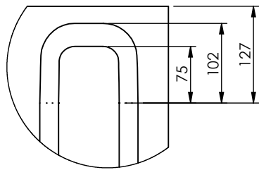
DETAIL B SCALE 1 : 7
