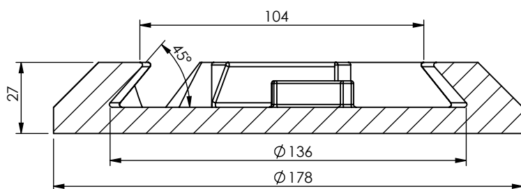
Section C-C SCALE 1 : 2
