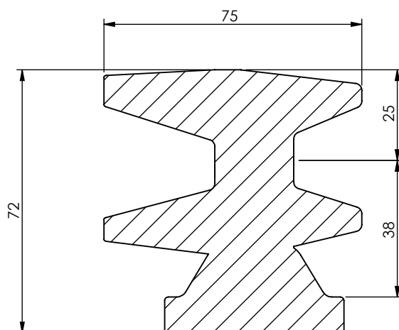
SECTION C-C SCALE 1 : 1.5
