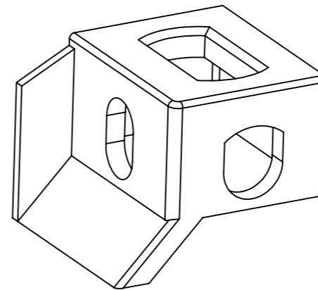
Top corner casting left (B) (Top right configuration is the mirrored version)
