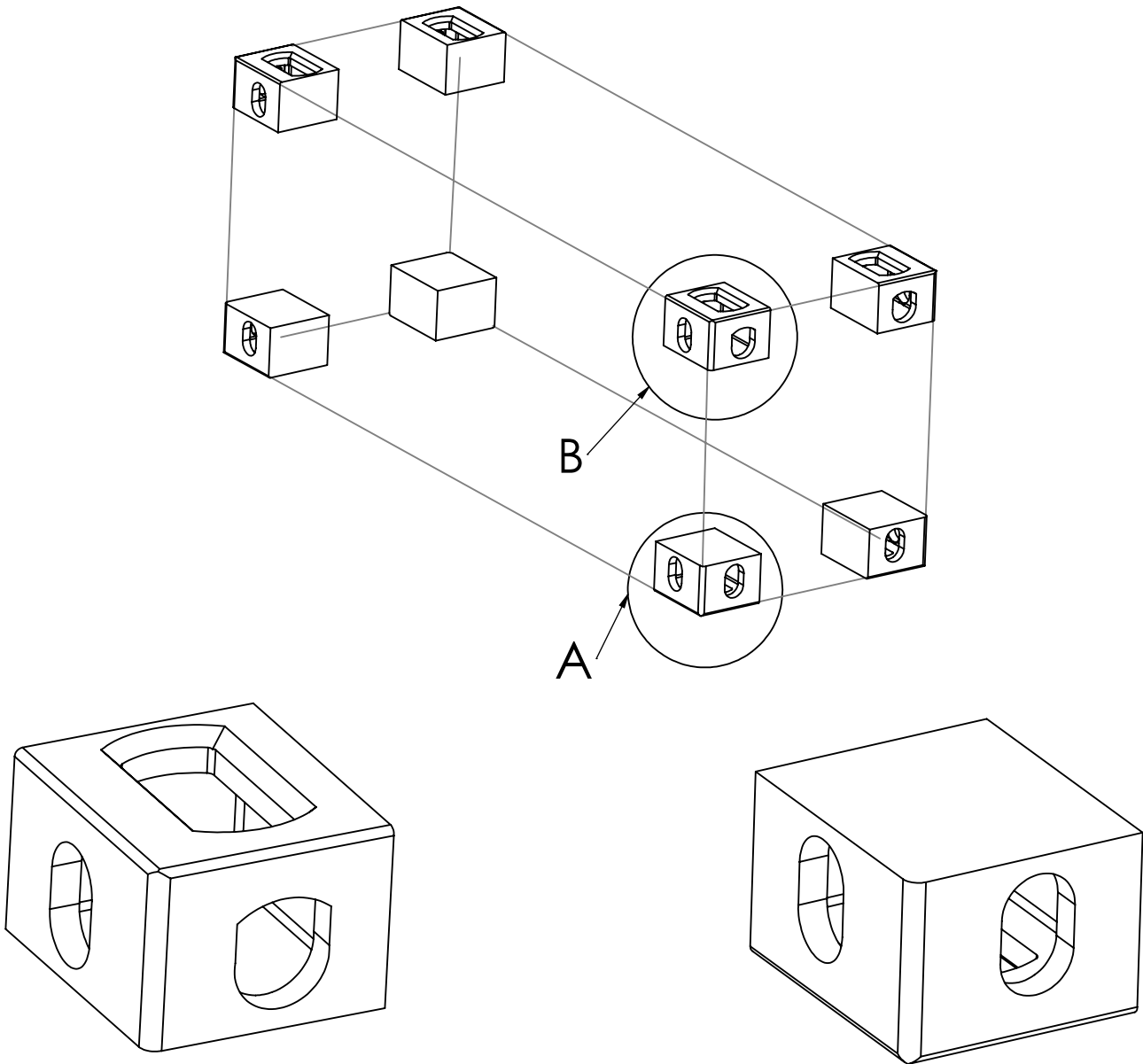
Top corner fitting left (B) (Top right configuratoin is the mirrored version)
